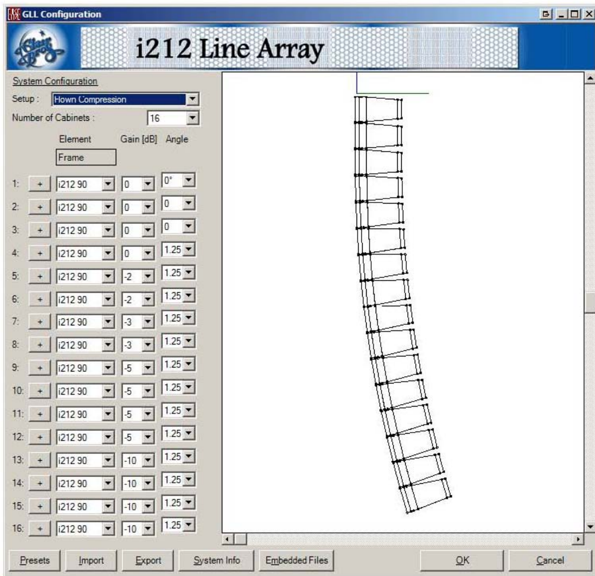
Figure 1.2.2 – Stage Left Cluster Configuration: Front center of top grid located at x=38\text{ft} , y=-10\text{ft} , z=44\text{ft} (relative to origin). Top grid is angled down 6.0 degrees.
