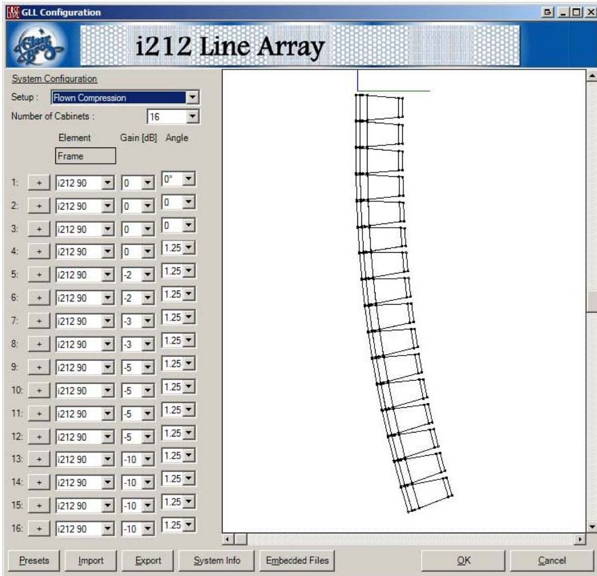
Figure 1.2.3 – Stage Right Cluster Configuration: Front center of top grid located at x = -29.53\text{ft} , y = 2\text{ft} , z = 44\text{ft} (relative to origin). Top grid is angled down 6.0 degrees.
